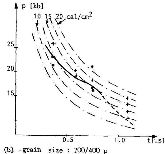
Fig 6 Sensitivity of Granular RDX
